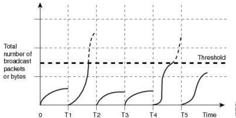
Figure 18: Broadcast Suppression
